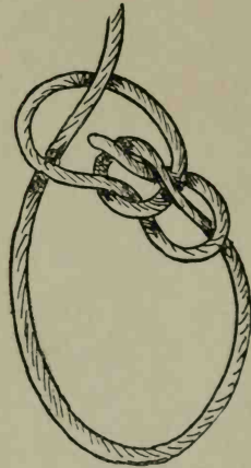
FIG. 60.—Bow-line on bight. FIG. 61.—Running bow-line.
